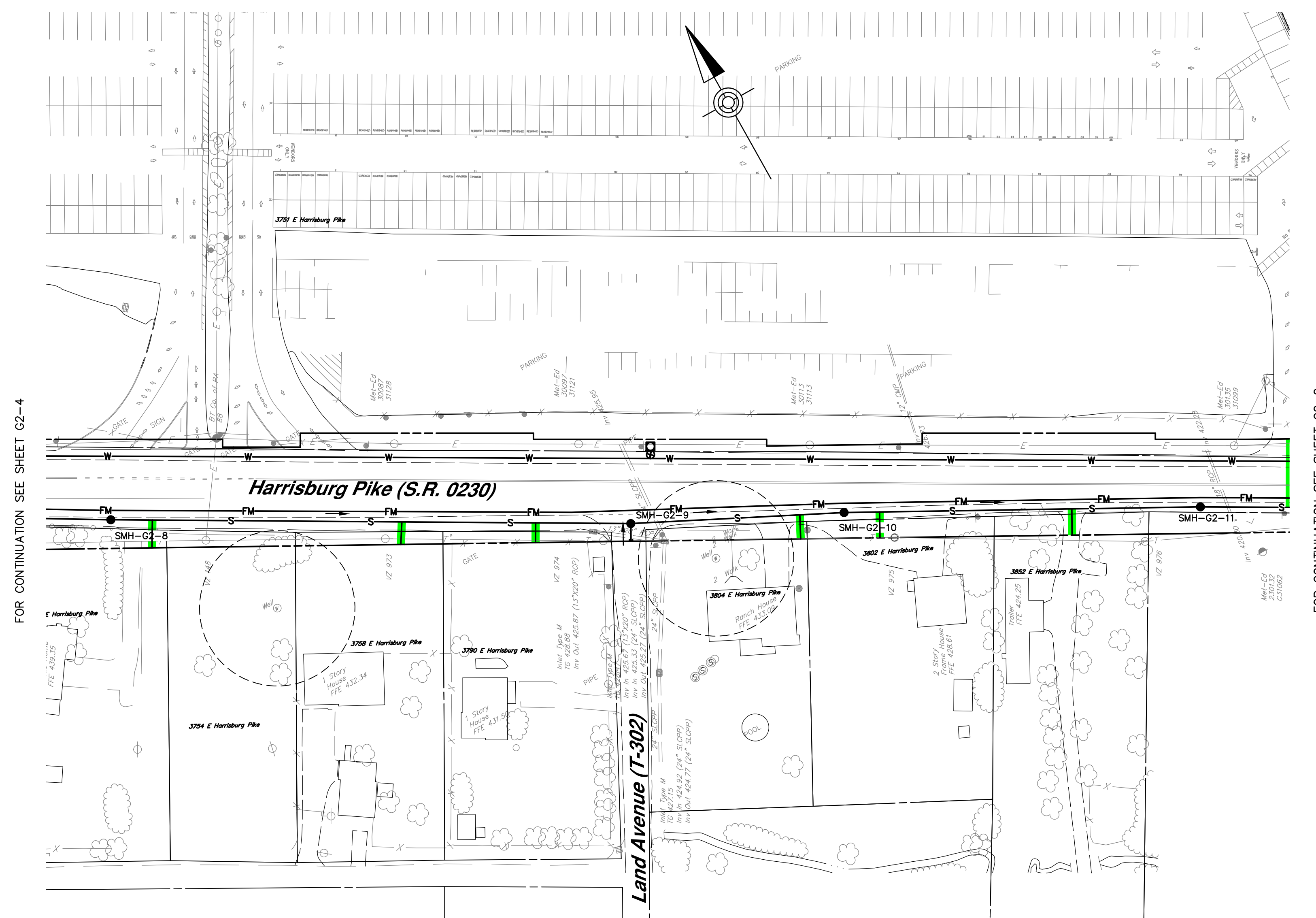
SANITARY SEWER PLAN SCALE: 1" = 50'
