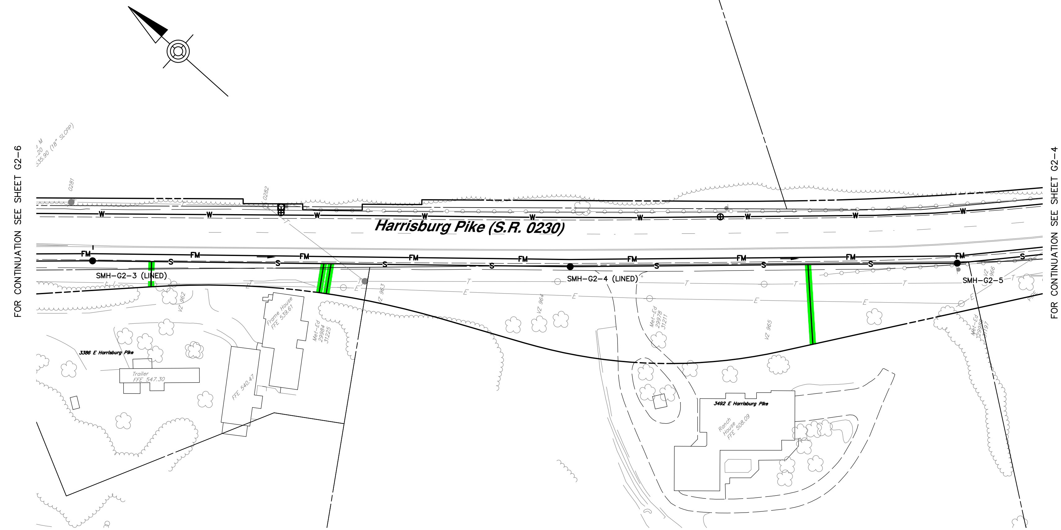
SANITARY SEWER PLAN SCALE: 1" = 50'
