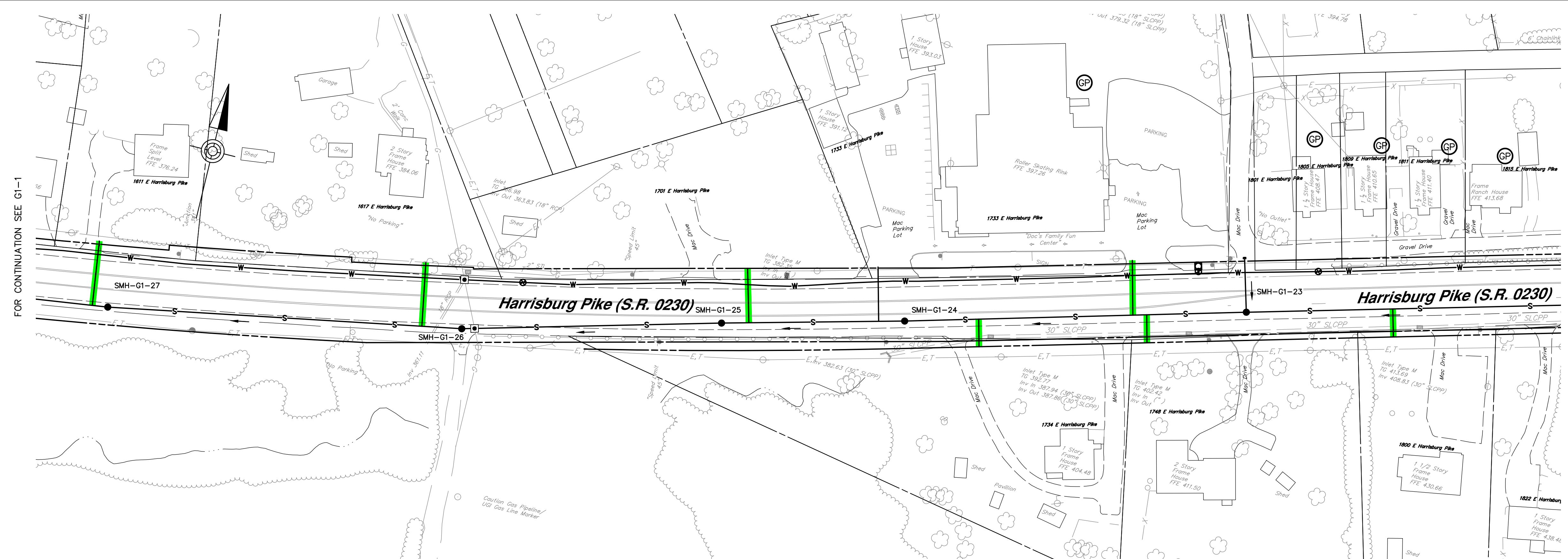
SANITARY SEWER PLAN SCALE: 1" = 50'
